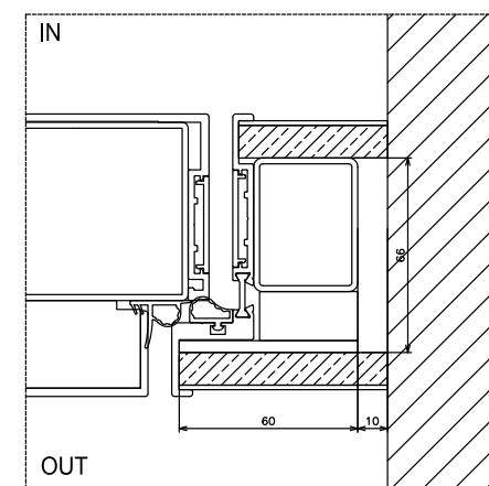
- Detail 1 - Wall connection
