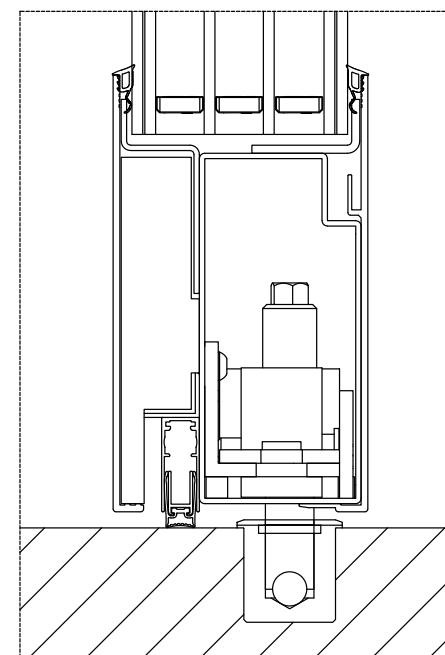
- Detail 2 - Floor section
